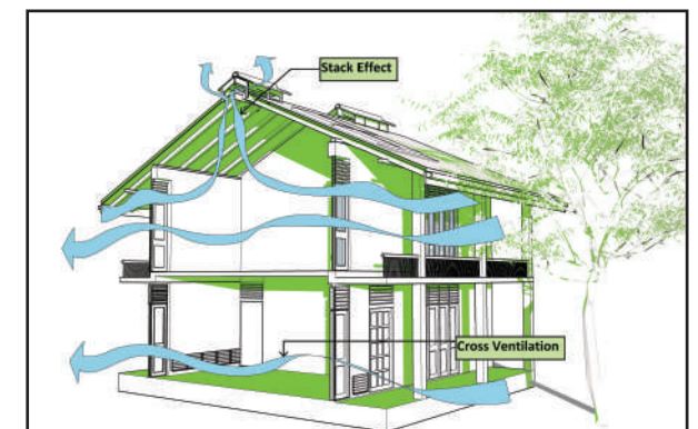
Fig | 22: Types of Ventilation
