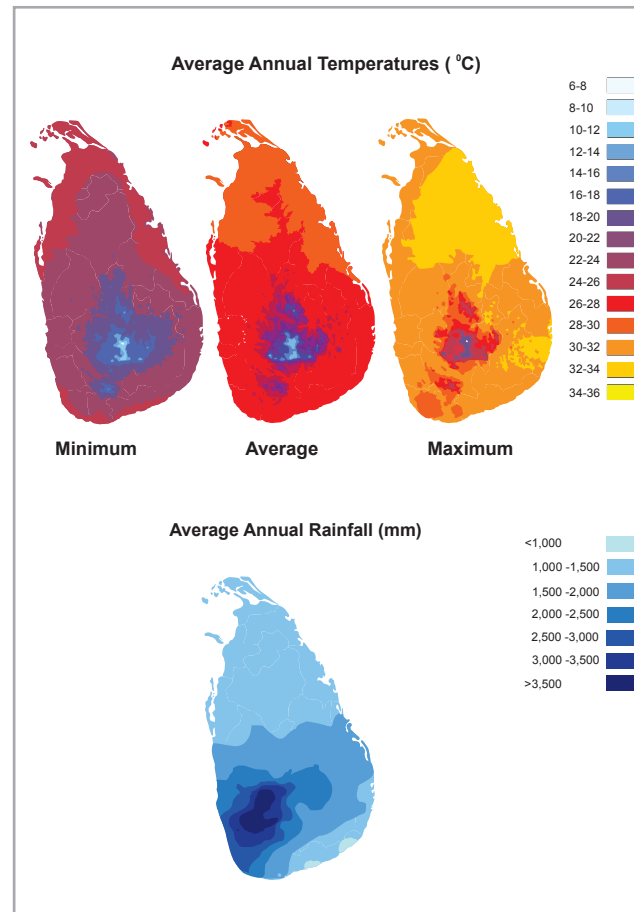
Fig | 1: Average Annual Temperature and Rainfall- Sri Lanka
