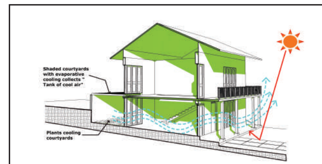
Fig | 25: Cool Courtyard – Pergola Shaded, Vegetated and /or Water Surface
