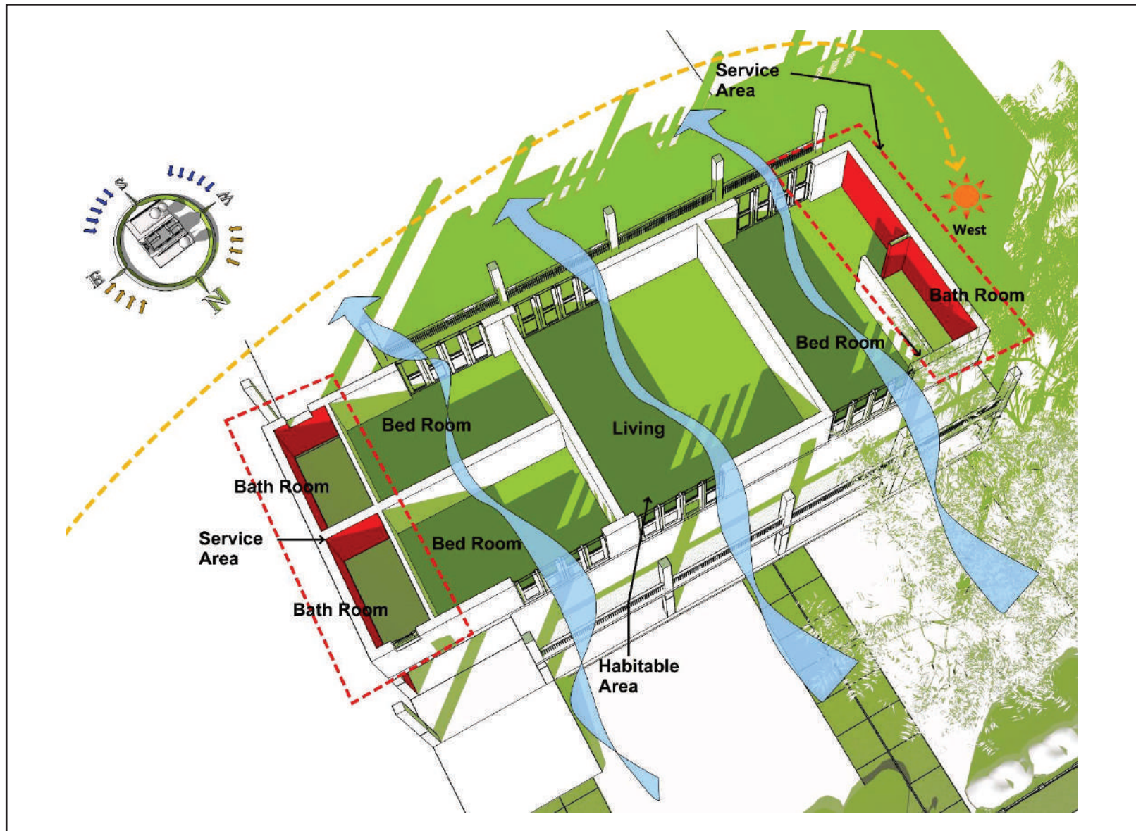
Fig | 55: Plan Form - First Floor Two Storey Residence
