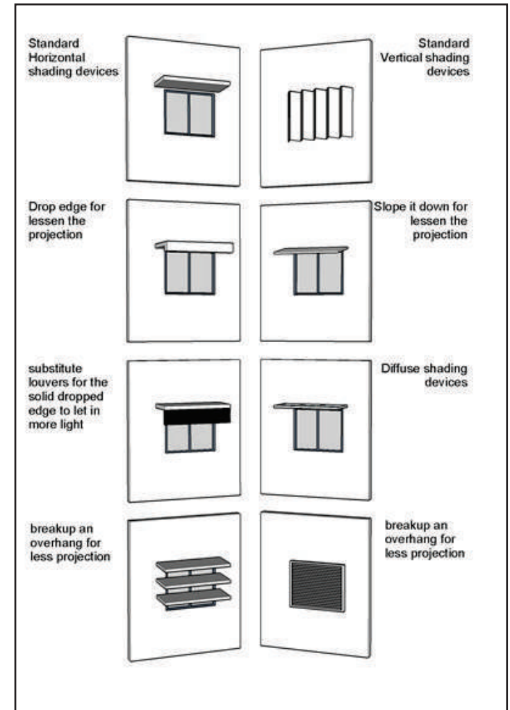
Fig | 19: Provide Shading for Glazing exposed to Sun
